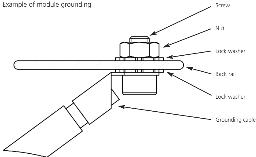
Example of module grounding
